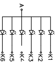
BACKLIGHT CIRCUIT DIAGRAM 120mA/LED (6LED)
